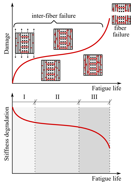
Typical fatigue damage evolution process of FRP composites
